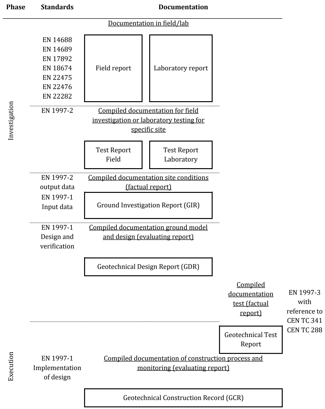
Figure C.1 Illustration of interaction between documentation in EN 1997 and complementary European standards.
